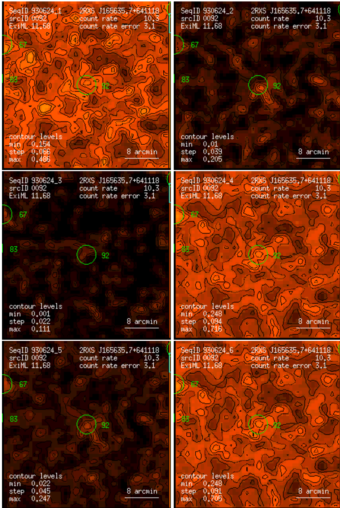
Figure 92: RASS 930624: detection 0092: band rate images, Gaussian filter: (1) PSPC channels 11 – 41, (2) 52 – 90, (3) 91 – 201, (4) 11 – 235, (5) 52 – 201, (6) 11 – 201. Broad band rates in counts/ks. Band rate contour levels in counts/ks/arcmin 2 .
