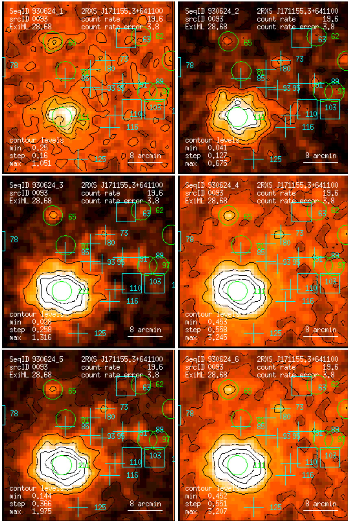
Figure 93: RASS 930624: detection 0093: band rate images, Gaussian filter: (1) PSPC channels 11 – 41, (2) 52 – 90, (3) 91 – 201, (4) 11 – 235, (5) 52 – 201, (6) 11 – 201. Broad band rates in counts/ks. Band rate contour levels in counts/ks/arcmin 2 .
