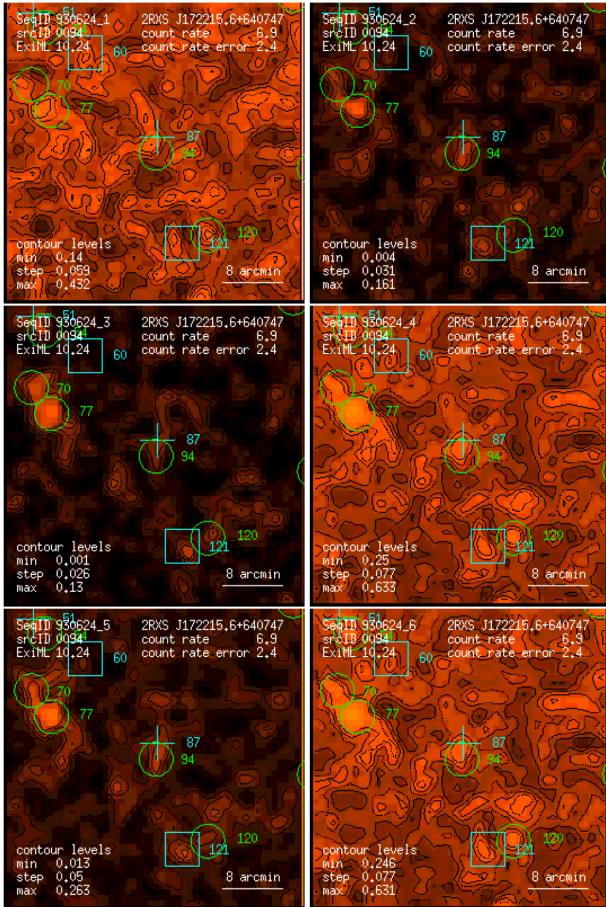
Figure 94: RASS 930624: detection 0094: band rate images, Gaussian filter: (1) PSPC channels 11 – 41, (2) 52 – 90, (3) 91 – 201, (4) 11 – 235, (5) 52 – 201, (6) 11 – 201. Broad band rates in counts/ks. Band rate contour levels in counts/ks/arcmin 2 .
