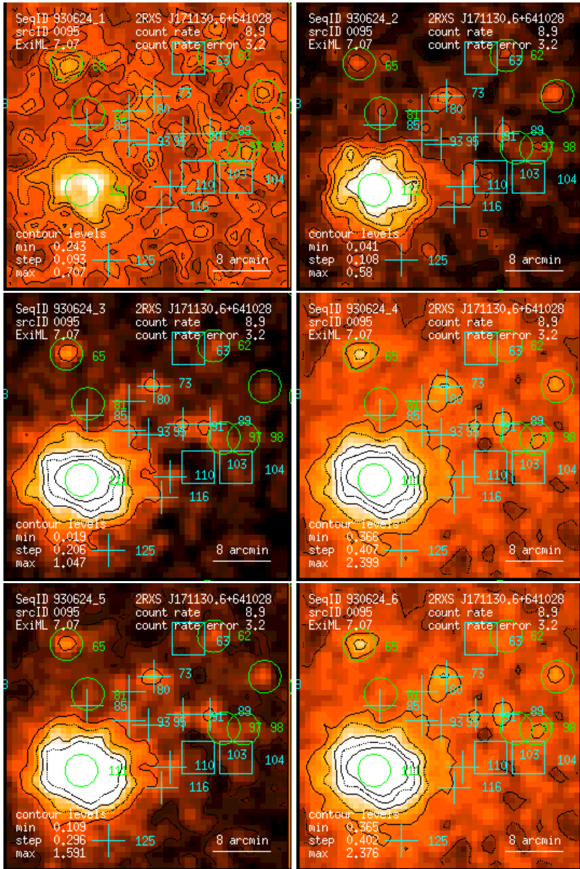
Figure 95: RASS 930624: detection 0095: band rate images, Gaussian filter: (1) PSPC channels 11 – 41, (2) 52 – 90, (3) 91 – 201, (4) 11 – 235, (5) 52 – 201, (6) 11 – 201. Broad band rates in counts/ks. Band rate contour levels in counts/ks/arcmin 2 .
