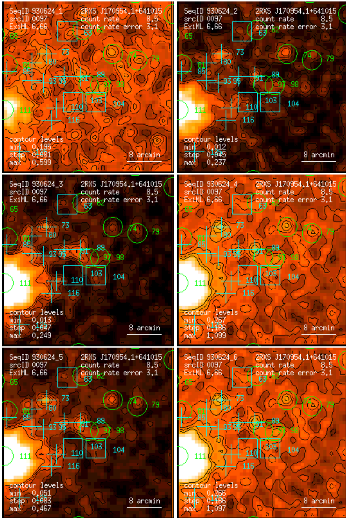
Figure 97: RASS 930624: detection 0097: band rate images, Gaussian filter: (1) PSPC channels 11 – 41, (2) 52 – 90, (3) 91 – 201, (4) 11 – 235, (5) 52 – 201, (6) 11 – 201. Broad band rates in counts/ks. Band rate contour levels in counts/ks/arcmin 2 .
