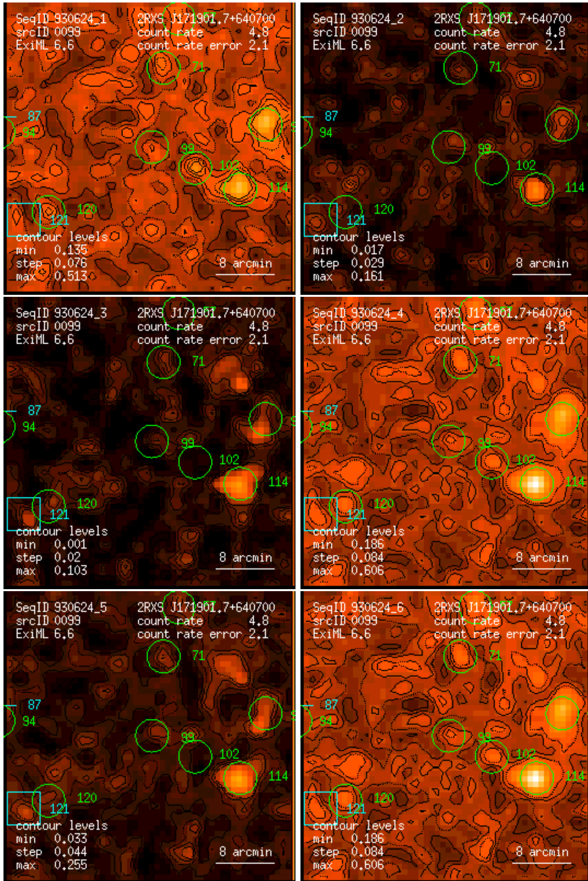
Figure 99: RASS 930624: detection 0099: band rate images, Gaussian filter: (1) PSPC channels 11 – 41, (2) 52 – 90, (3) 91 – 201, (4) 11 – 235, (5) 52 – 201, (6) 11 – 201. Broad band rates in counts/ks. Band rate contour levels in counts/ks/arcmin 2 .
