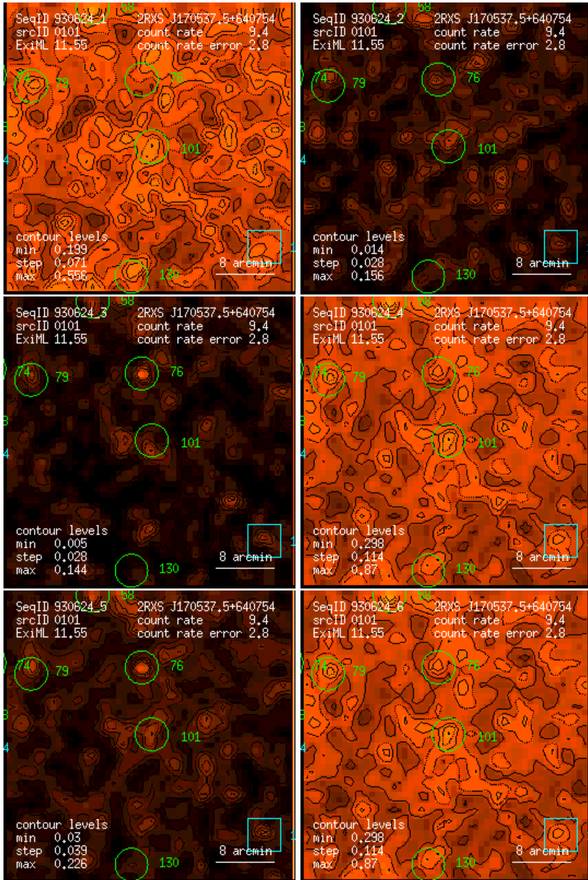
Figure 101: RASS 930624: detection 0101: band rate images, Gaussian filter: (1) PSPC channels 11 – 41, (2) 52 – 90, (3) 91 – 201, (4) 11 – 235, (5) 52 – 201, (6) 11 – 201. Broad band rates in counts/ks. Band rate contour levels in counts/ks/arcmin 2 .
