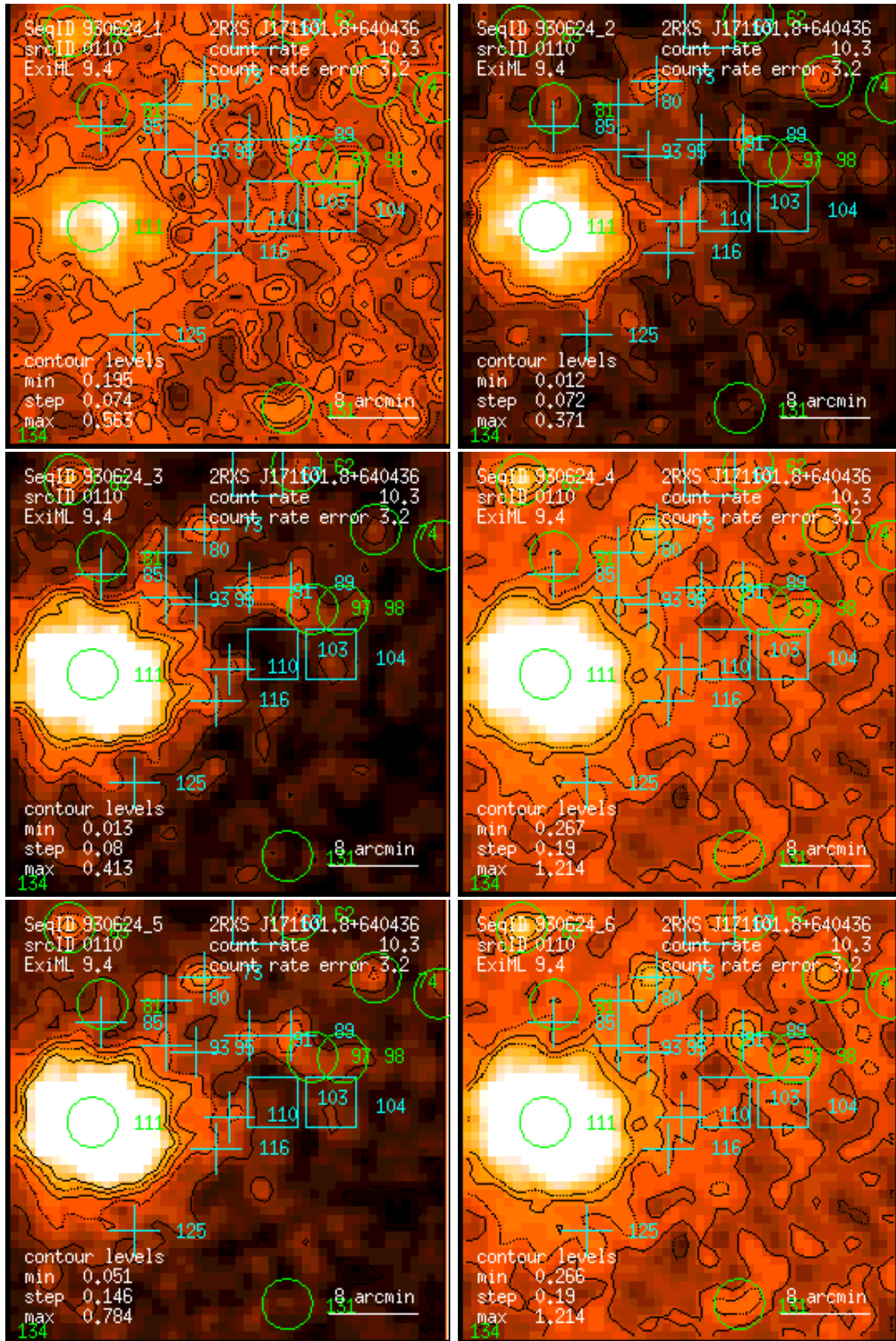
Figure 110: RASS 930624: detection 0110: band rate images, Gaussian filter: (1) PSPC channels 11 – 41, (2) 52 – 90, (3) 91 – 201, (4) 11 – 235, (5) 52 – 201, (6) 11 – 201. Broad band rates in counts/ks. Band rate contour levels in counts/ks/arcmin 2 .
