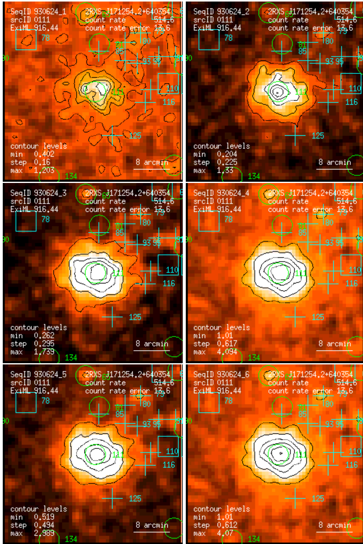
Figure 111: RASS 930624: detection 0111: band rate images, Gaussian filter: (1) PSPC channels 11 – 41, (2) 52 – 90, (3) 91 – 201, (4) 11 – 235, (5) 52 – 201, (6) 11 – 201. Broad band rates in counts/ks. Band rate contour levels in counts/ks/arcmin 2 .
