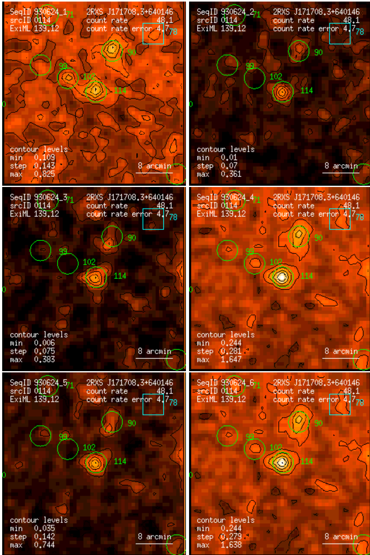
Figure 114: RASS 930624: detection 0114: band rate images, Gaussian filter: (1) PSPC channels 11 – 41, (2) 52 – 90, (3) 91 – 201, (4) 11 – 235, (5) 52 – 201, (6) 11 – 201. Broad band rates in counts/ks. Band rate contour levels in counts/ks/arcmin 2 .
