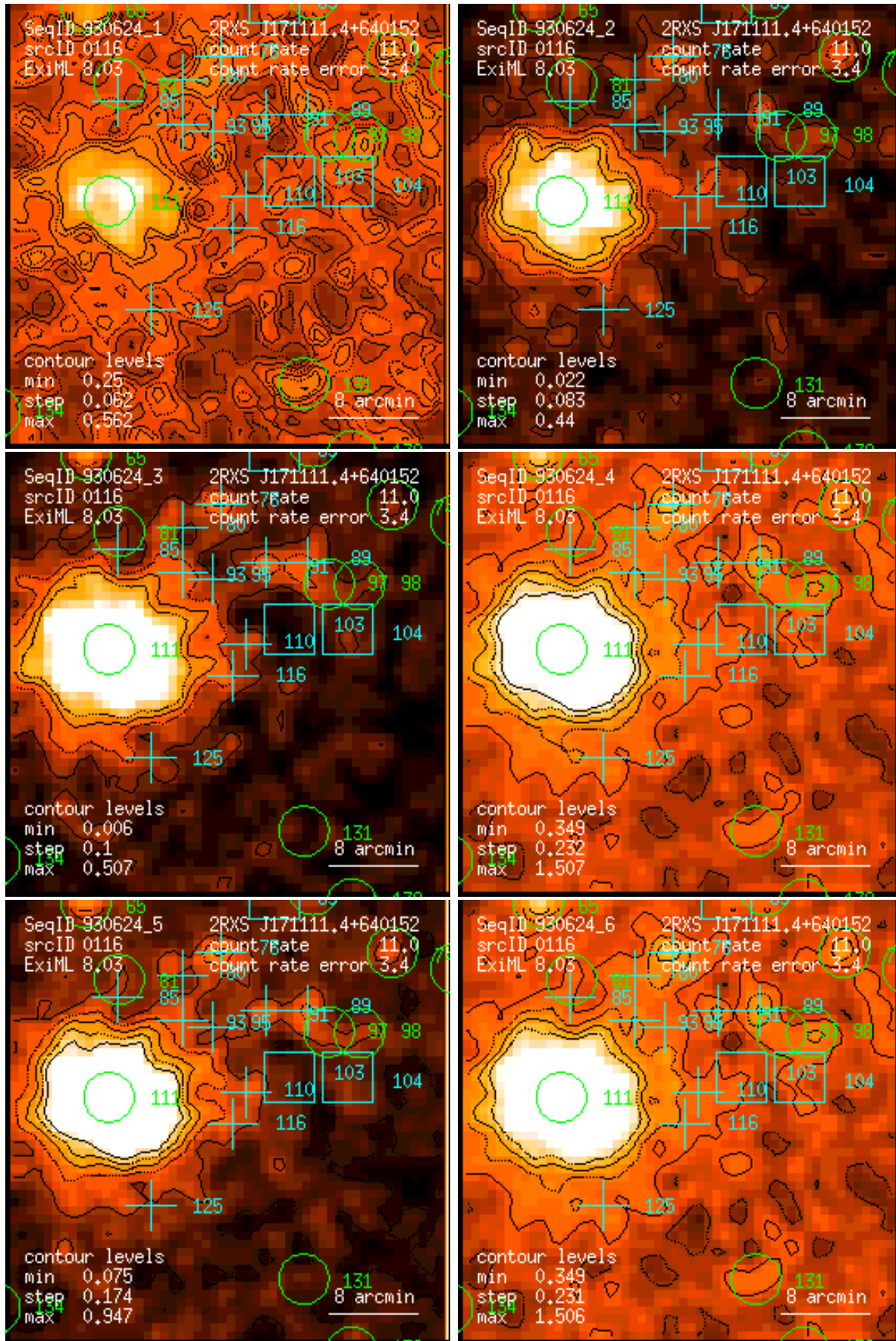
Figure 116: RASS 930624: detection 0116: band rate images, Gaussian filter: (1) PSPC channels 11 – 41, (2) 52 – 90, (3) 91 – 201, (4) 11 – 235, (5) 52 – 201, (6) 11 – 201. Broad band rates in counts/ks. Band rate contour levels in counts/ks/arcmin 2 .
