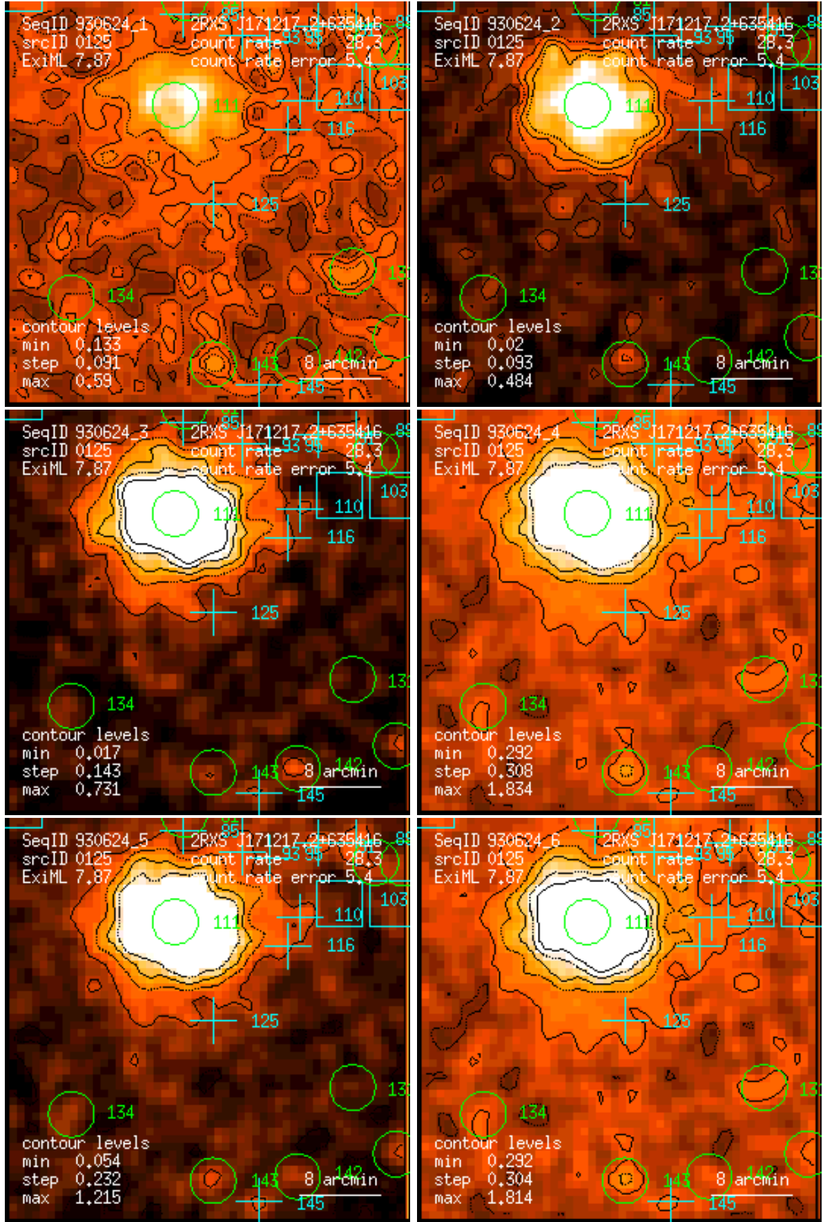
Figure 125: RASS 930624: detection 0125: band rate images, Gaussian filter: (1) PSPC channels 11 – 41, (2) 52 – 90, (3) 91 – 201, (4) 11 – 235, (5) 52 – 201, (6) 11 – 201. Broad band rates in counts/ks. Band rate contour levels in counts/ks/arcmin 2 .
