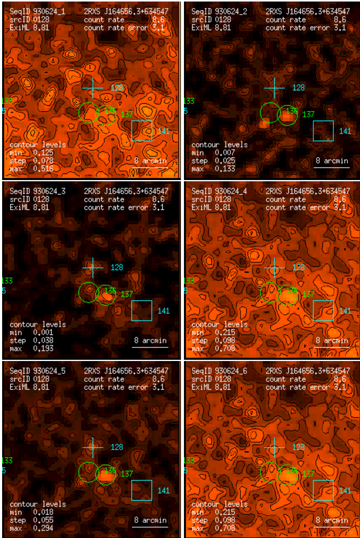
Figure 128: RASS 930624: detection 0128: band rate images, Gaussian filter: (1) PSPC channels 11 – 41, (2) 52 – 90, (3) 91 – 201, (4) 11 – 235, (5) 52 – 201, (6) 11 – 201. Broad band rates in counts/ks. Band rate contour levels in counts/ks/arcmin 2 .
