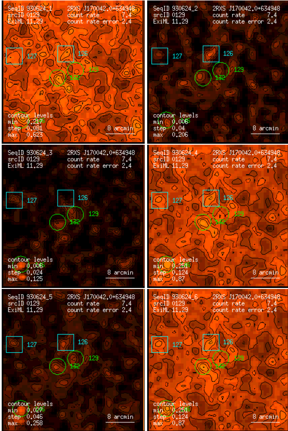
Figure 129: RASS 930624: detection 0129: band rate images, Gaussian filter: (1) PSPC channels 11 – 41, (2) 52 – 90, (3) 91 – 201, (4) 11 – 235, (5) 52 – 201, (6) 11 – 201. Broad band rates in counts/ks. Band rate contour levels in counts/ks/arcmin 2 .
