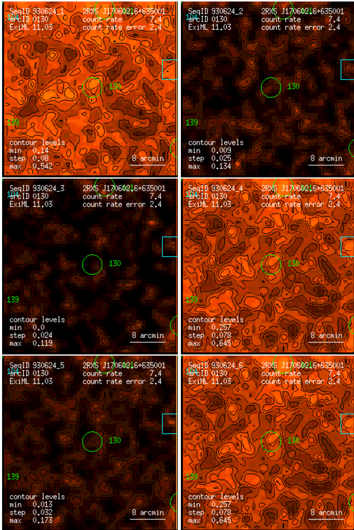
Figure 130: RASS 930624: detection 0130: band rate images, Gaussian filter: (1) PSPC channels 11 – 41, (2) 52 – 90, (3) 91 – 201, (4) 11 – 235, (5) 52 – 201, (6) 11 – 201. Broad band rates in counts/ks. Band rate contour levels in counts/ks/arcmin 2 .
