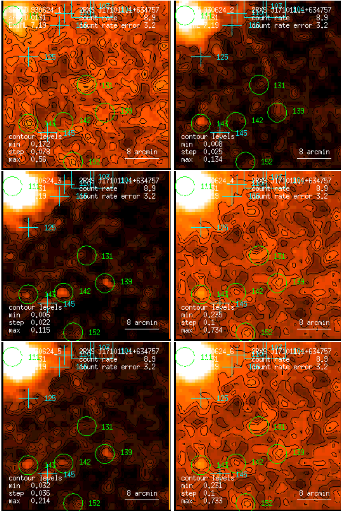
Figure 131: RASS 930624: detection 0131: band rate images, Gaussian filter: (1) PSPC channels 11 – 41, (2) 52 – 90, (3) 91 – 201, (4) 11 – 235, (5) 52 – 201, (6) 11 – 201. Broad band rates in counts/ks. Band rate contour levels in counts/ks/arcmin 2 .
