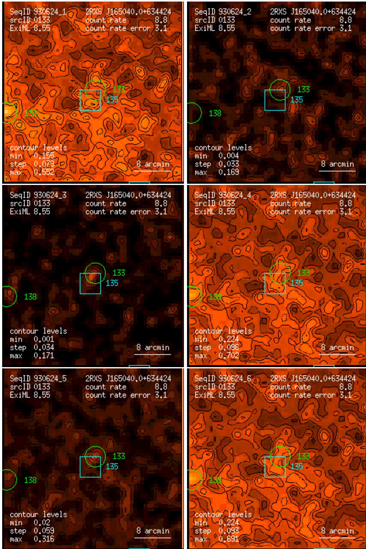
Figure 133: RASS 930624: detection 0133: band rate images, Gaussian filter: (1) PSPC channels 11 – 41, (2) 52 – 90, (3) 91 – 201, (4) 11 – 235, (5) 52 – 201, (6) 11 – 201. Broad band rates in counts/ks. Band rate contour levels in counts/ks/arcmin 2 .
