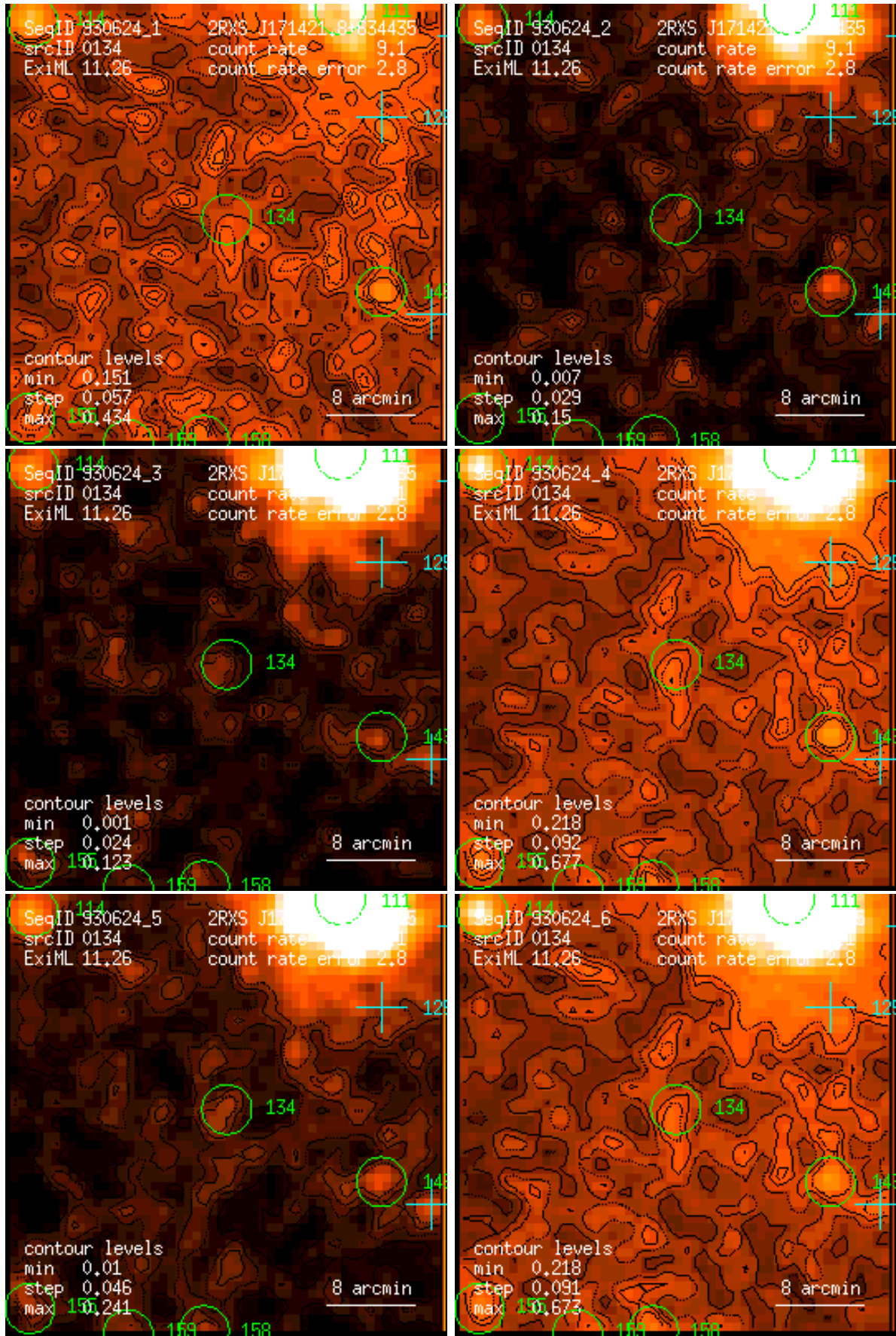
Figure 134: RASS 930624: detection 0134: band rate images, Gaussian filter: (1) PSPC channels 11 – 41, (2) 52 – 90, (3) 91 – 201, (4) 11 – 235, (5) 52 – 201, (6) 11 – 201. Broad band rates in counts/ks. Band rate contour levels in counts/ks/arcmin 2 .
