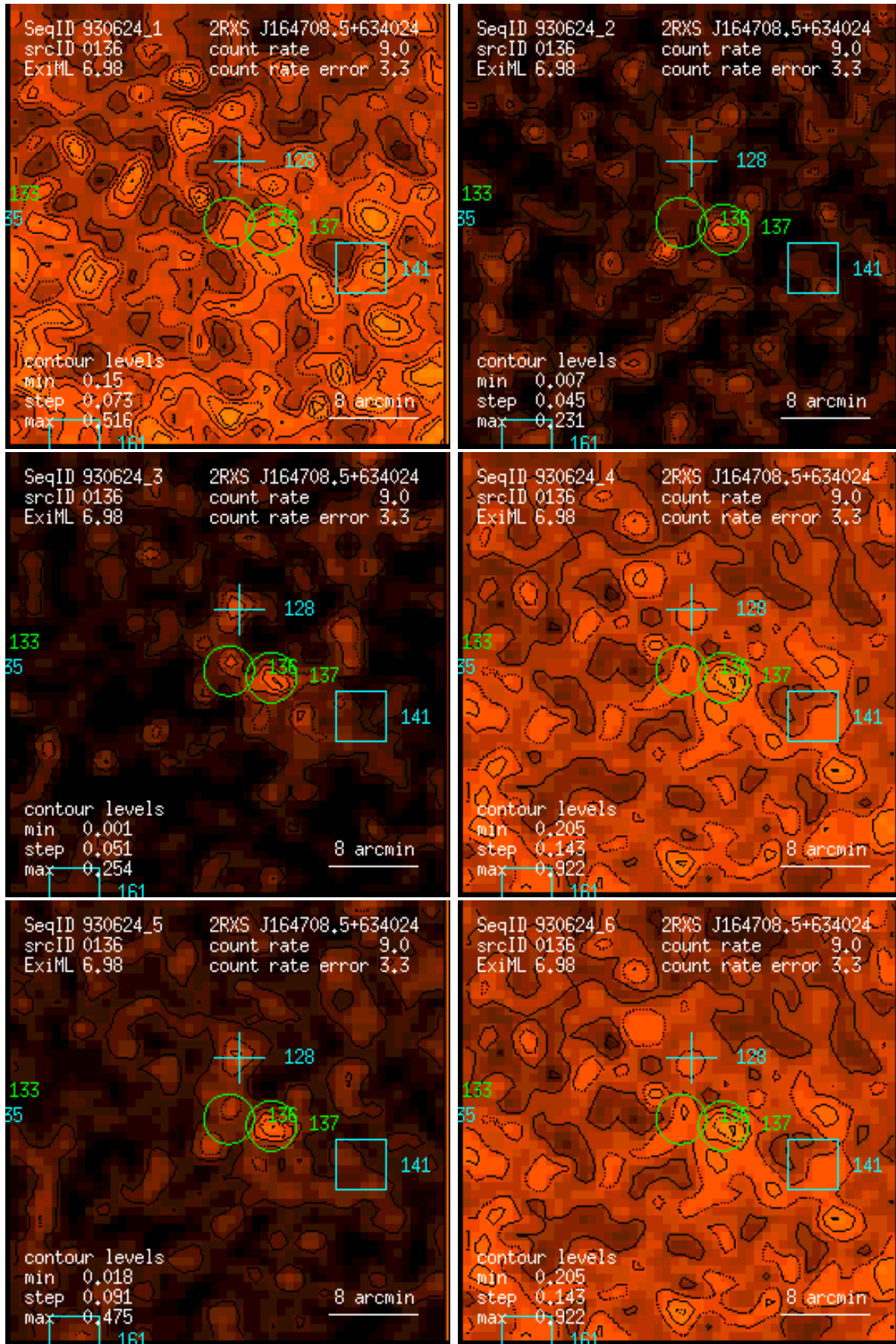
Figure 136: RASS 930624: detection 0136: band rate images, Gaussian filter: (1) PSPC channels 11 – 41, (2) 52 – 90, (3) 91 – 201, (4) 11 – 235, (5) 52 – 201, (6) 11 – 201. Broad band rates in counts/ks. Band rate contour levels in counts/ks/arcmin 2 .
