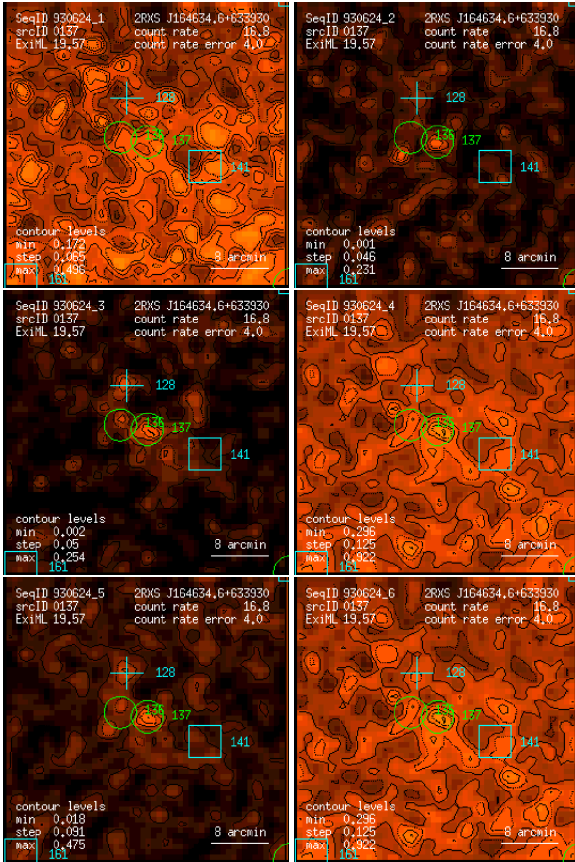
Figure 137: RASS 930624: detection 0137: band rate images, Gaussian filter: (1) PSPC channels 11 – 41, (2) 52 – 90, (3) 91 – 201, (4) 11 – 235, (5) 52 – 201, (6) 11 – 201. Broad band rates in counts/ks. Band rate contour levels in counts/ks/arcmin 2 .
