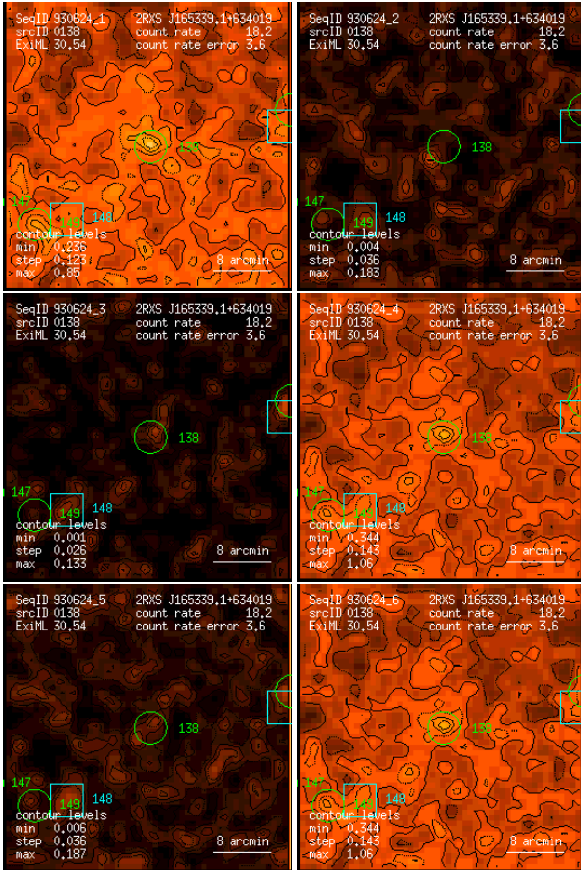
Figure 138: RASS 930624: detection 0138: band rate images, Gaussian filter: (1) PSPC channels 11 – 41, (2) 52 – 90, (3) 91 – 201, (4) 11 – 235, (5) 52 – 201, (6) 11 – 201. Broad band rates in counts/ks. Band rate contour levels in counts/ks/arcmin 2 .
