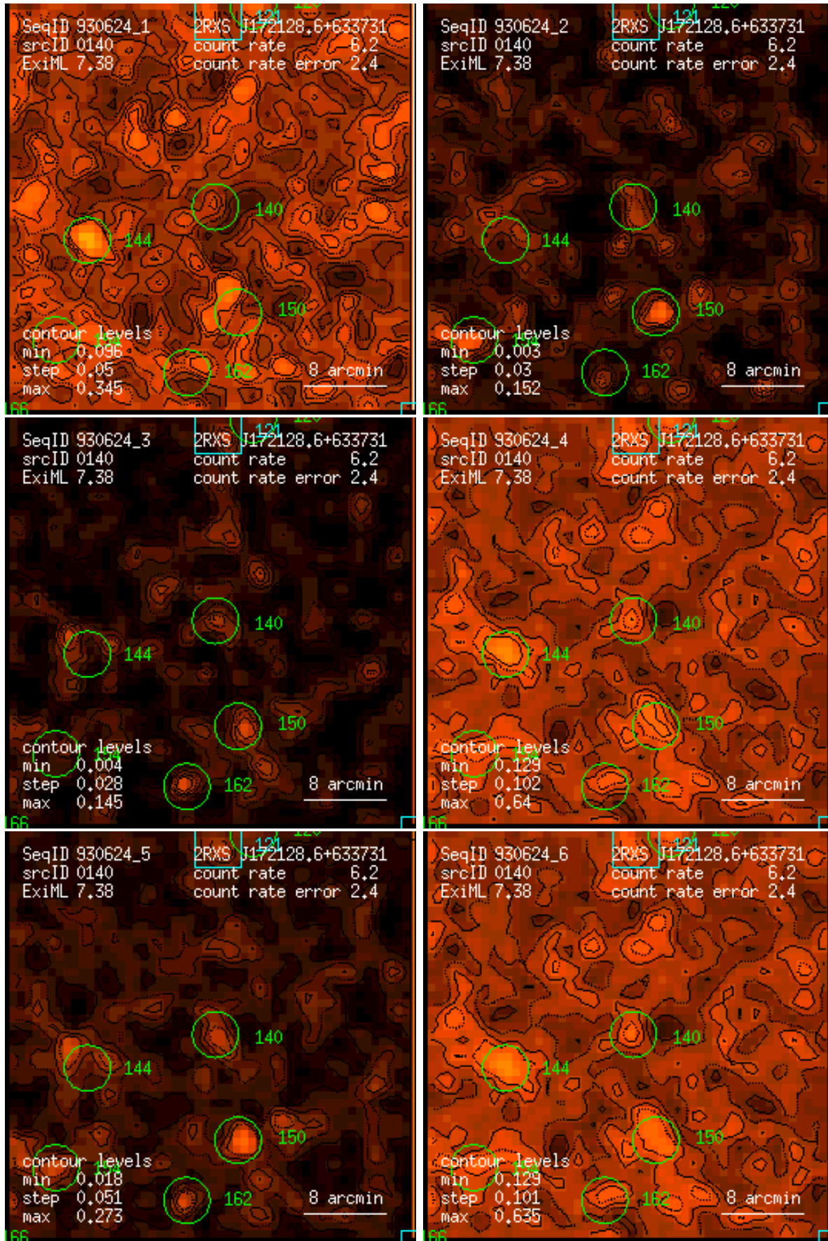
Figure 140: RASS 930624: detection 0140: band rate images, Gaussian filter: (1) PSPC channels 11 – 41, (2) 52 – 90, (3) 91 – 201, (4) 11 – 235, (5) 52 – 201, (6) 11 – 201. Broad band rates in counts/ks. Band rate contour levels in counts/ks/arcmin 2 .
