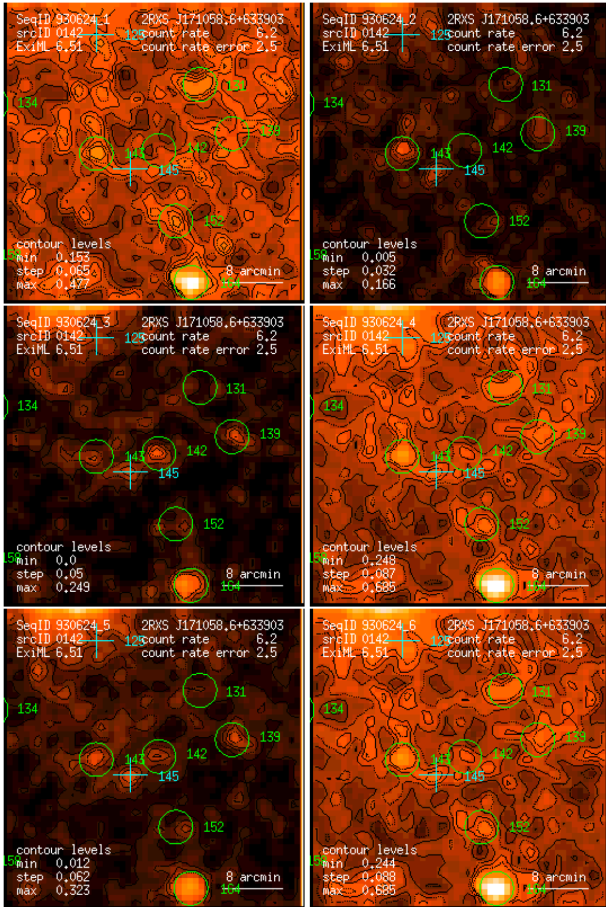
Figure 142: RASS 930624: detection 0142: band rate images, Gaussian filter: (1) PSPC channels 11 – 41, (2) 52 – 90, (3) 91 – 201, (4) 11 – 235, (5) 52 – 201, (6) 11 – 201. Broad band rates in counts/ks. Band rate contour levels in counts/ks/arcmin 2 .
