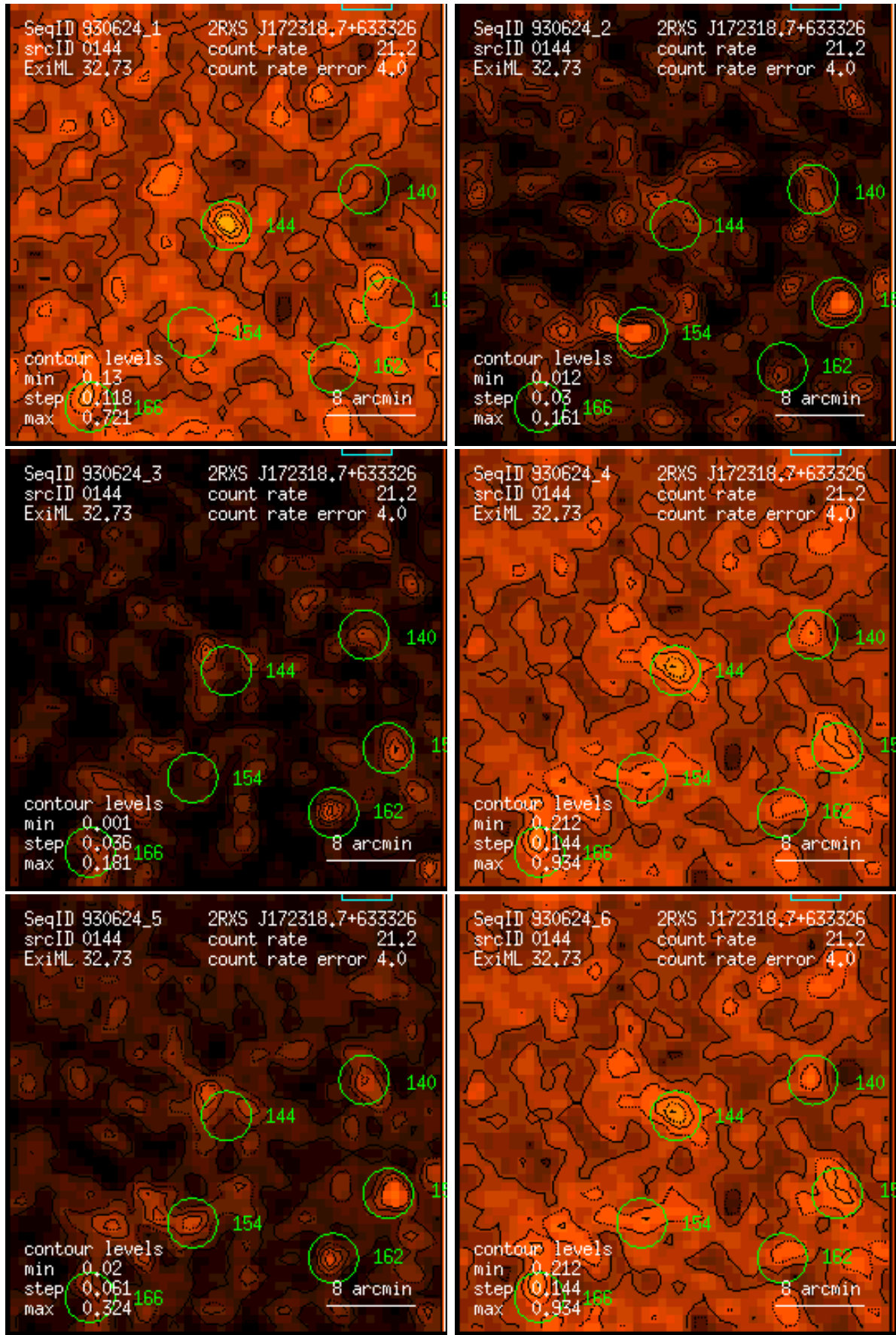
Figure 144: RASS 930624: detection 0144: band rate images, Gaussian filter: (1) PSPC channels 11 – 41, (2) 52 – 90, (3) 91 – 201, (4) 11 – 235, (5) 52 – 201, (6) 11 – 201. Broad band rates in counts/ks. Band rate contour levels in counts/ks/arcmin 2 .
