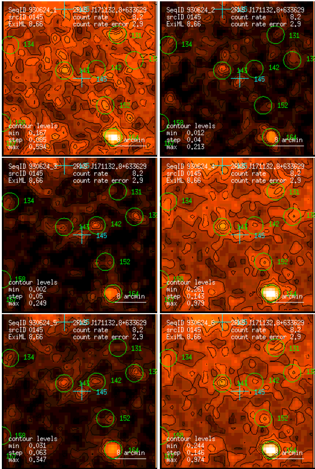
Figure 145: RASS 930624: detection 0145: band rate images, Gaussian filter: (1) PSPC channels 11 – 41, (2) 52 – 90, (3) 91 – 201, (4) 11 – 235, (5) 52 – 201, (6) 11 – 201. Broad band rates in counts/ks. Band rate contour levels in counts/ks/arcmin 2 .
