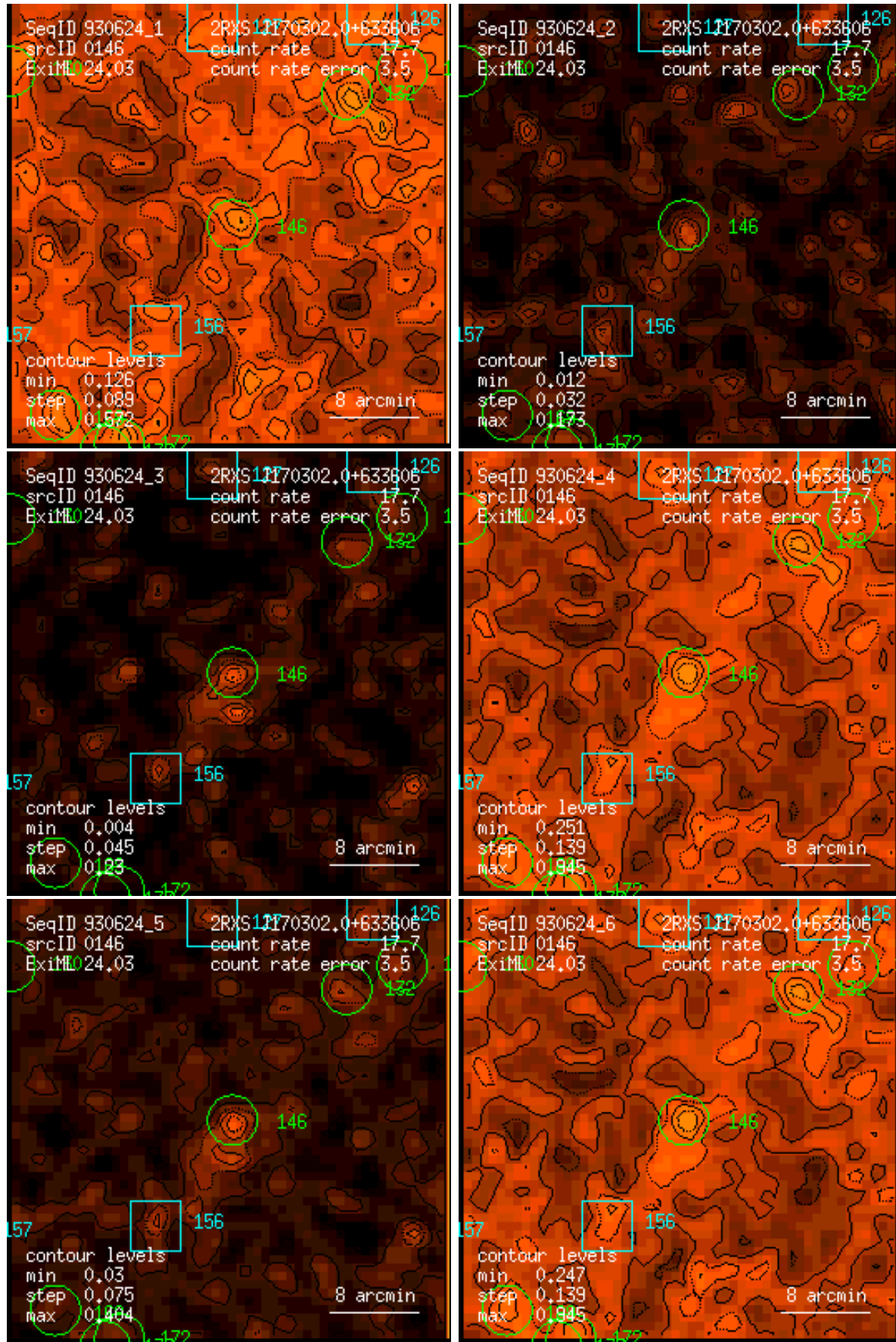
Figure 146: RASS 930624: detection 0146: band rate images, Gaussian filter: (1) PSPC channels 11 – 41, (2) 52 – 90, (3) 91 – 201, (4) 11 – 235, (5) 52 – 201, (6) 11 – 201. Broad band rates in counts/ks. Band rate contour levels in counts/ks/arcmin 2 .
