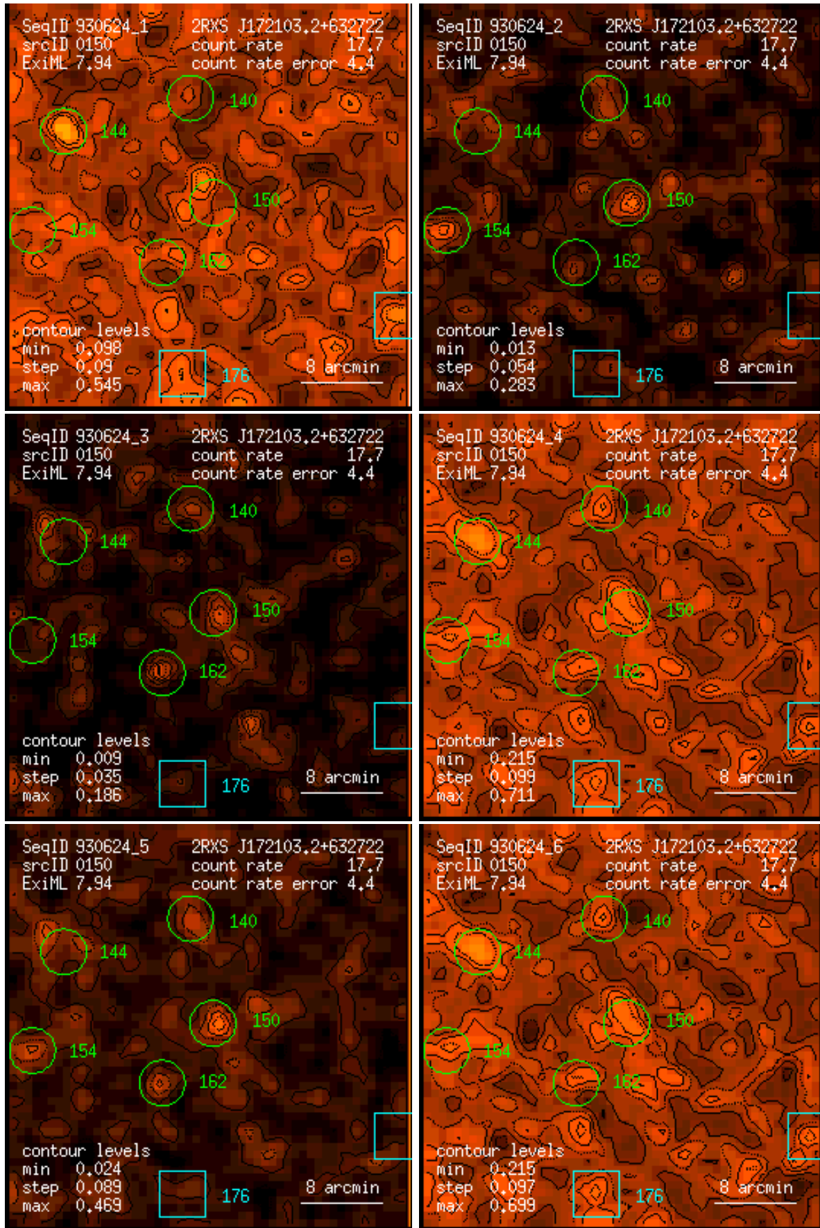
Figure 150: RASS 930624: detection 0150: band rate images, Gaussian filter: (1) PSPC channels 11 – 41, (2) 52 – 90, (3) 91 – 201, (4) 11 – 235, (5) 52 – 201, (6) 11 – 201. Broad band rates in counts/ks. Band rate contour levels in counts/ks/arcmin 2 .
