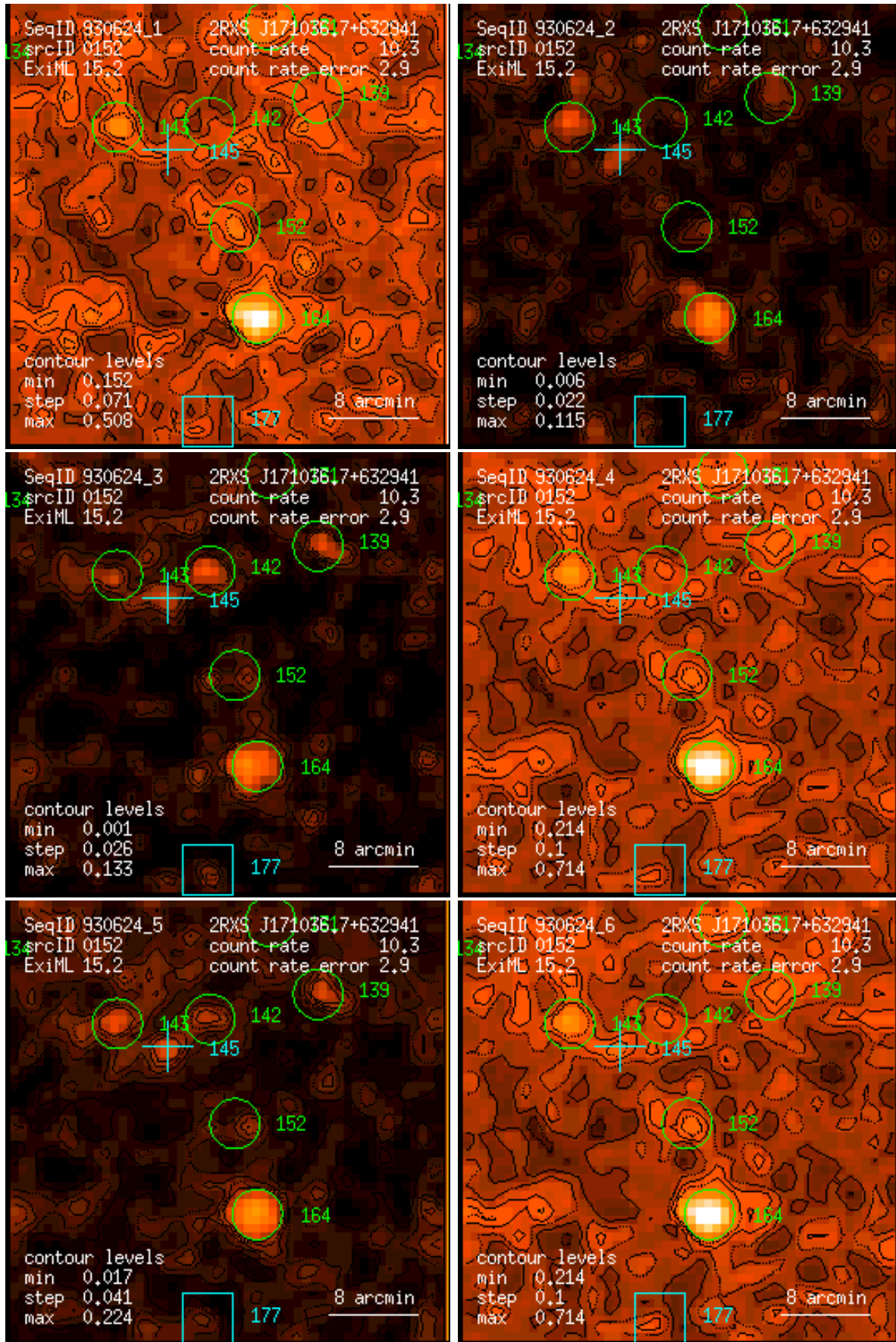
Figure 152: RASS 930624: detection 0152: band rate images, Gaussian filter: (1) PSPC channels 11 – 41, (2) 52 – 90, (3) 91 – 201, (4) 11 – 235, (5) 52 – 201, (6) 11 – 201. Broad band rates in counts/ks. Band rate contour levels in counts/ks/arcmin 2 .
