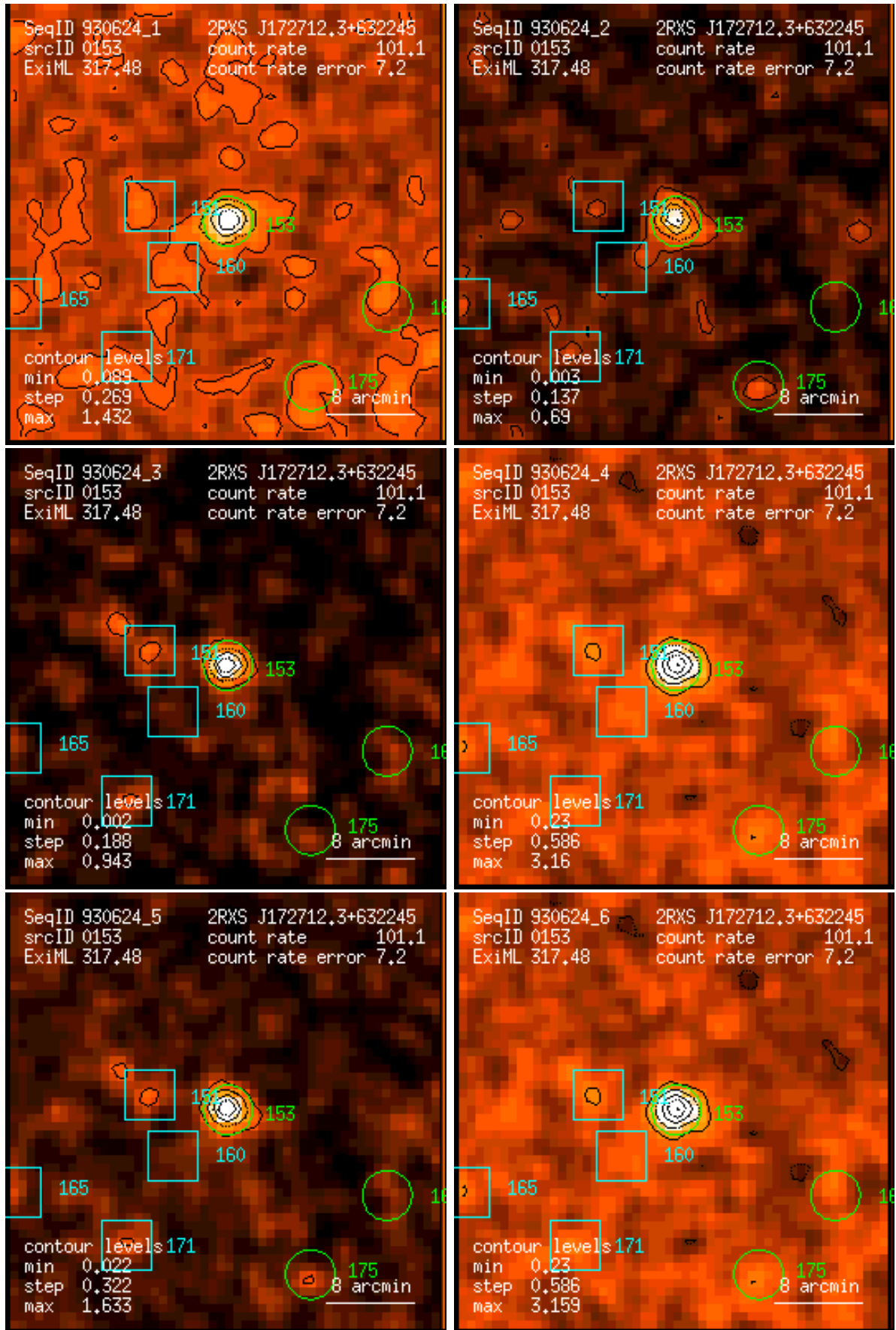
Figure 153: RASS 930624: detection 0153: band rate images, Gaussian filter: (1) PSPC channels 11 – 41, (2) 52 – 90, (3) 91 – 201, (4) 11 – 235, (5) 52 – 201, (6) 11 – 201. Broad band rates in counts/ks. Band rate contour levels in counts/ks/arcmin 2 .
