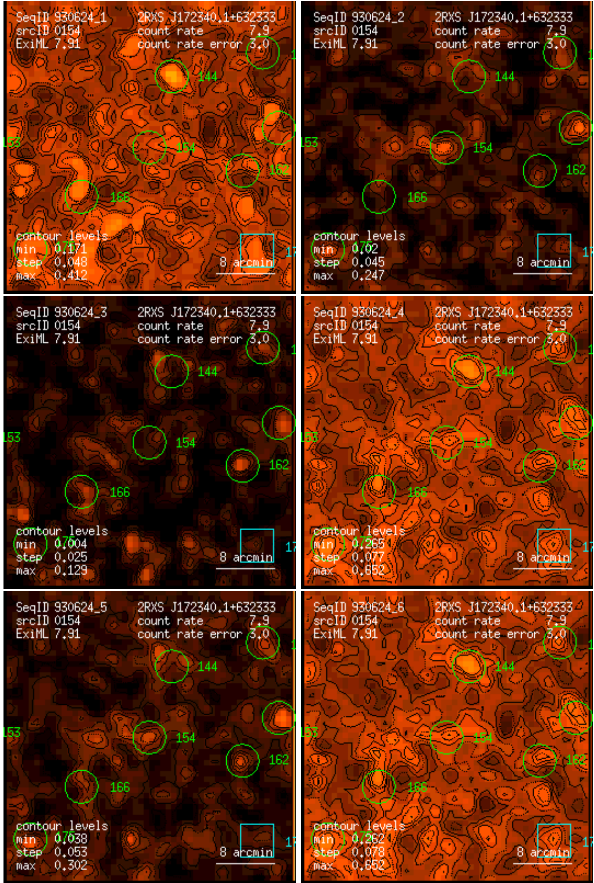
Figure 154: RASS 930624: detection 0154: band rate images, Gaussian filter: (1) PSPC channels 11 – 41, (2) 52 – 90, (3) 91 – 201, (4) 11 – 235, (5) 52 – 201, (6) 11 – 201. Broad band rates in counts/ks. Band rate contour levels in counts/ks/arcmin 2 .
