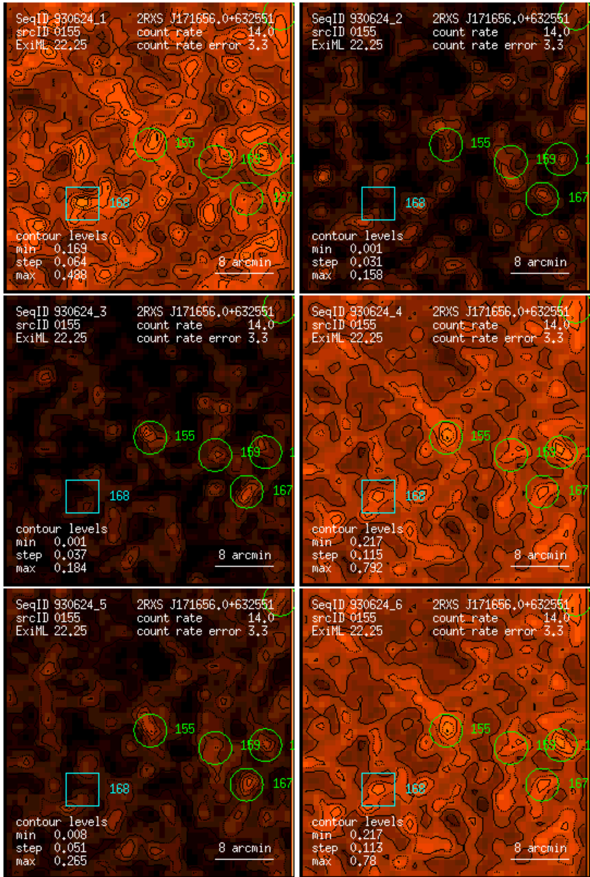
Figure 155: RASS 930624: detection 0155: band rate images, Gaussian filter: (1) PSPC channels 11 – 41, (2) 52 – 90, (3) 91 – 201, (4) 11 – 235, (5) 52 – 201, (6) 11 – 201. Broad band rates in counts/ks. Band rate contour levels in counts/ks/arcmin 2 .
