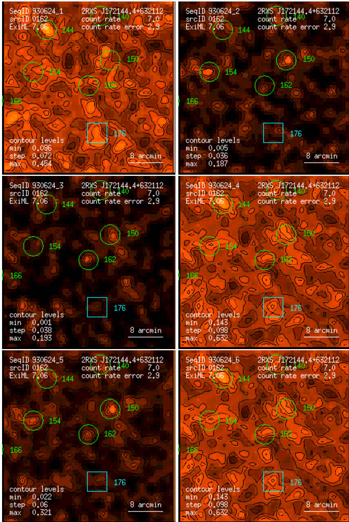
Figure 162: RASS 930624: detection 0162: band rate images, Gaussian filter: (1) PSPC channels 11 – 41, (2) 52 – 90, (3) 91 – 201, (4) 11 – 235, (5) 52 – 201, (6) 11 – 201. Broad band rates in counts/ks. Band rate contour levels in counts/ks/arcmin 2 .
