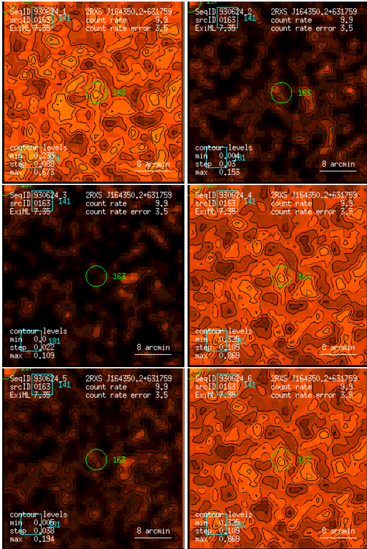
Figure 163: RASS 930624: detection 0163: band rate images, Gaussian filter: (1) PSPC channels 11 – 41, (2) 52 – 90, (3) 91 – 201, (4) 11 – 235, (5) 52 – 201, (6) 11 – 201. Broad band rates in counts/ks. Band rate contour levels in counts/ks/arcmin 2 .
