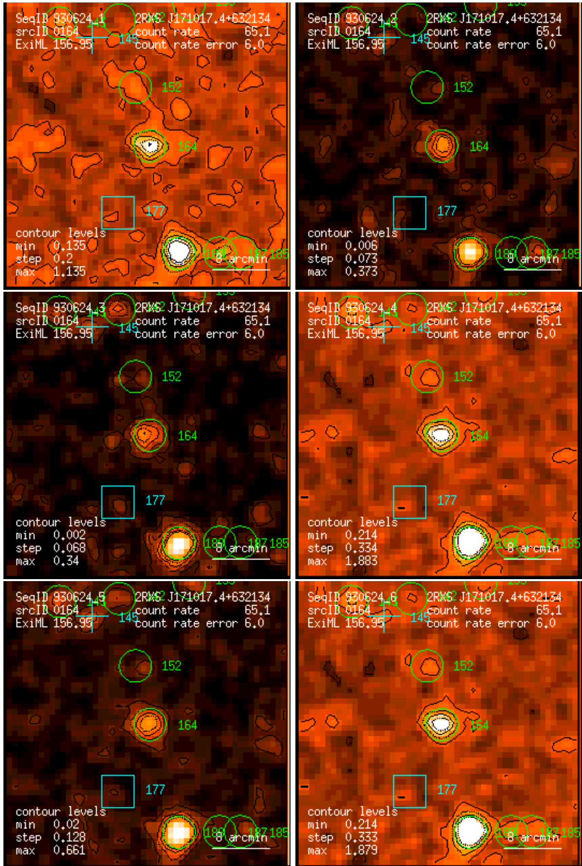
Figure 164: RASS 930624: detection 0164: band rate images, Gaussian filter: (1) PSPC channels 11 – 41, (2) 52 – 90, (3) 91 – 201, (4) 11 – 235, (5) 52 – 201, (6) 11 – 201. Broad band rates in counts/ks. Band rate contour levels in counts/ks/arcmin 2 .
