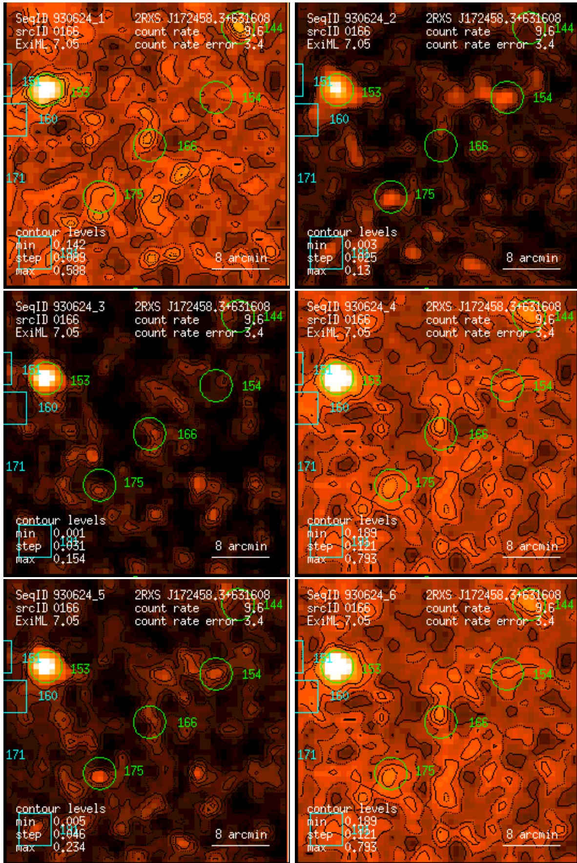
Figure 166: RASS 930624: detection 0166: band rate images, Gaussian filter: (1) PSPC channels 11 – 41, (2) 52 – 90, (3) 91 – 201, (4) 11 – 235, (5) 52 – 201, (6) 11 – 201. Broad band rates in counts/ks. Band rate contour levels in counts/ks/arcmin 2 .
