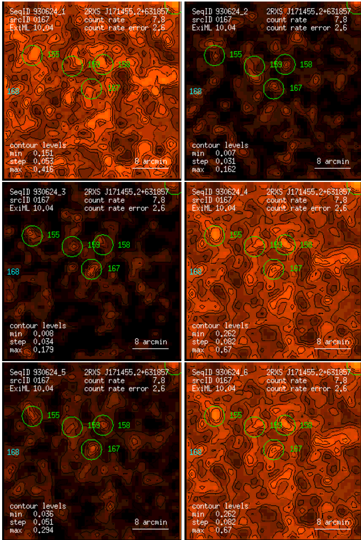
Figure 167: RASS 930624: detection 0167: band rate images, Gaussian filter: (1) PSPC channels 11 – 41, (2) 52 – 90, (3) 91 – 201, (4) 11 – 235, (5) 52 – 201, (6) 11 – 201. Broad band rates in counts/ks. Band rate contour levels in counts/ks/arcmin 2 .
