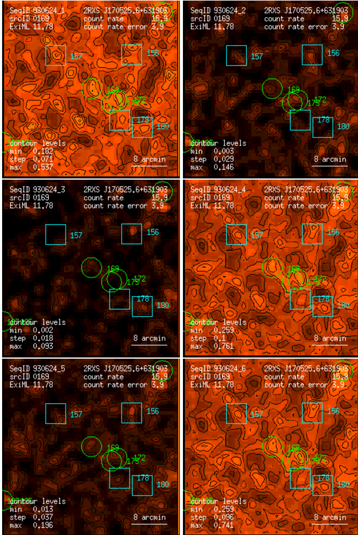
Figure 169: RASS 930624: detection 0169: band rate images, Gaussian filter: (1) PSPC channels 11 – 41, (2) 52 – 90, (3) 91 – 201, (4) 11 – 235, (5) 52 – 201, (6) 11 – 201. Broad band rates in counts/ks. Band rate contour levels in counts/ks/arcmin 2 .
