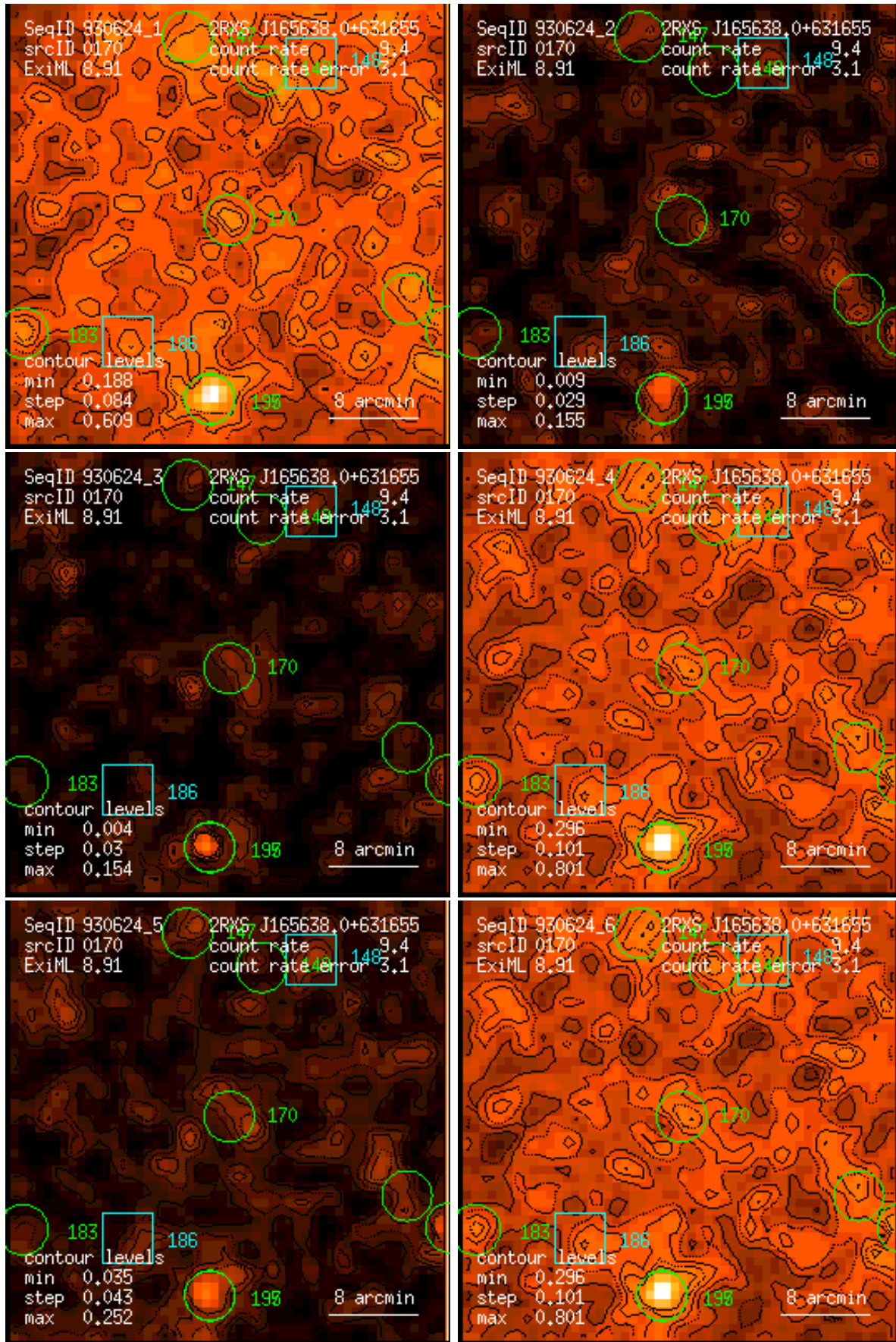
Figure 170: RASS 930624: detection 0170: band rate images, Gaussian filter: (1) PSPC channels 11 – 41, (2) 52 – 90, (3) 91 – 201, (4) 11 – 235, (5) 52 – 201, (6) 11 – 201. Broad band rates in counts/ks. Band rate contour levels in counts/ks/arcmin 2 .
