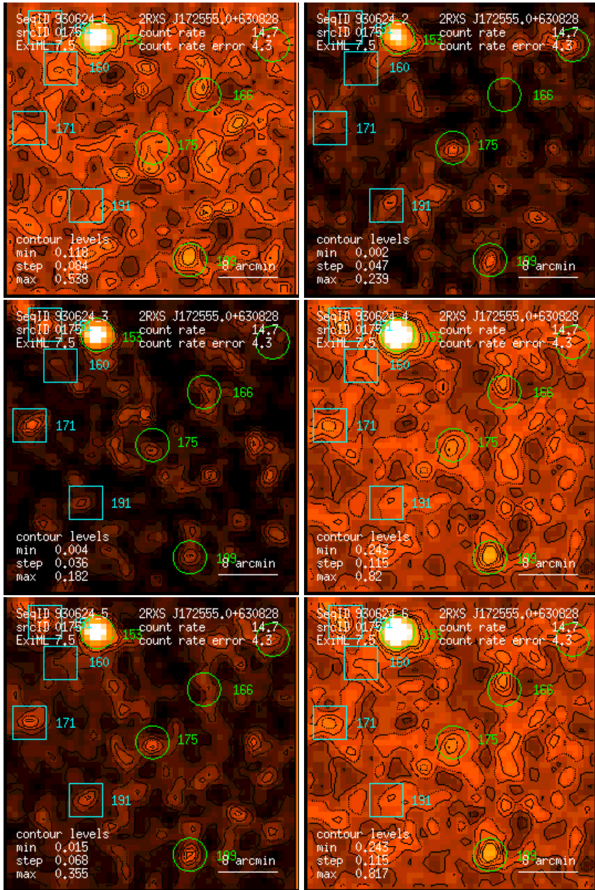
Figure 175: RASS 930624: detection 0175: band rate images, Gaussian filter: (1) PSPC channels 11 – 41, (2) 52 – 90, (3) 91 – 201, (4) 11 – 235, (5) 52 – 201, (6) 11 – 201. Broad band rates in counts/ks. Band rate contour levels in counts/ks/arcmin 2 .
