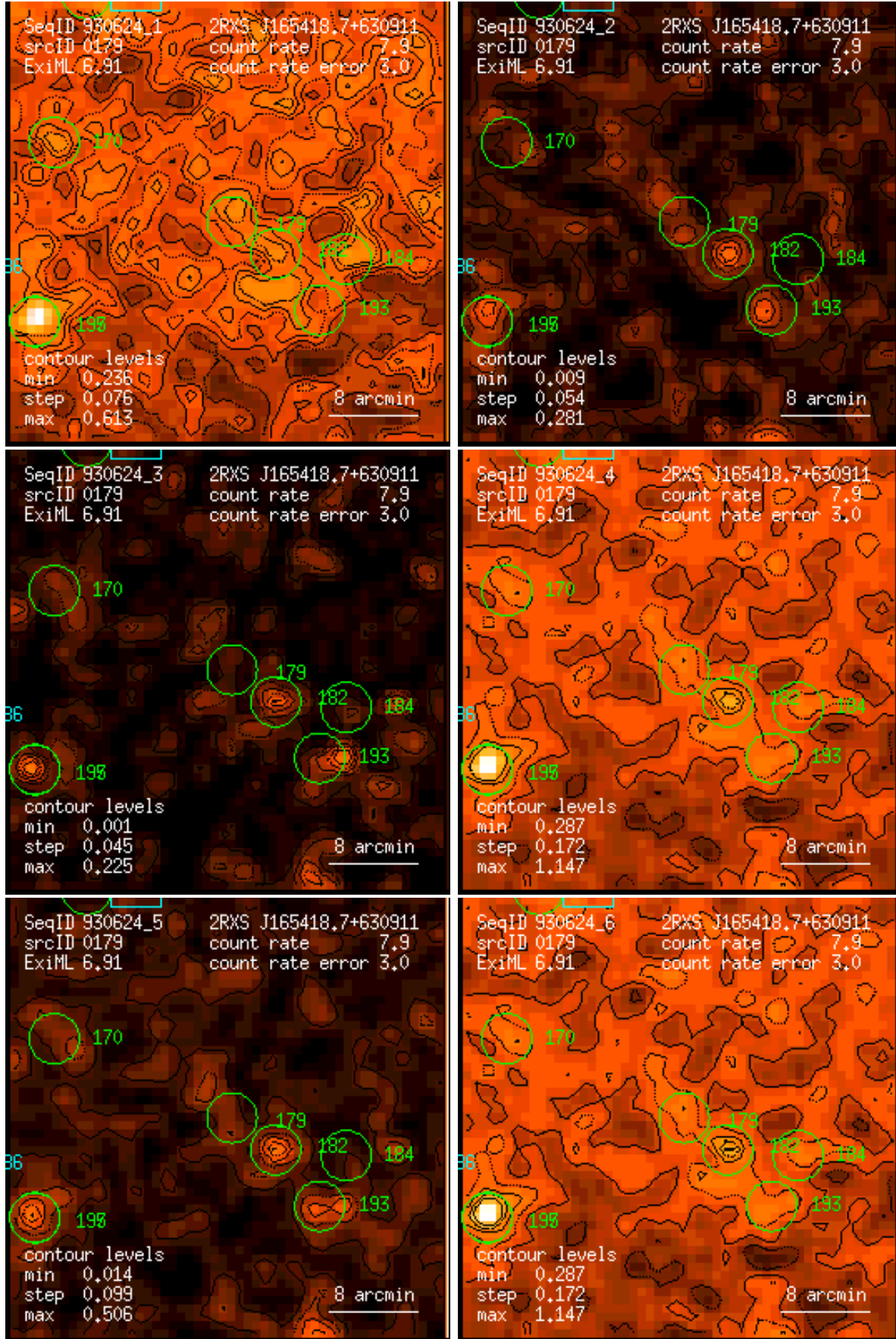
Figure 179: RASS 930624: detection 0179: band rate images, Gaussian filter: (1) PSPC channels 11 – 41, (2) 52 – 90, (3) 91 – 201, (4) 11 – 235, (5) 52 – 201, (6) 11 – 201. Broad band rates in counts/ks. Band rate contour levels in counts/ks/arcmin 2 .
