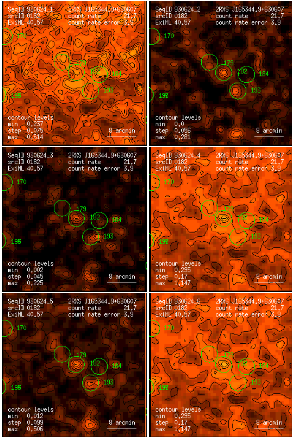
Figure 182: RASS 930624: detection 0182: band rate images, Gaussian filter: (1) PSPC channels 11 – 41, (2) 52 – 90, (3) 91 – 201, (4) 11 – 235, (5) 52 – 201, (6) 11 – 201. Broad band rates in counts/ks. Band rate contour levels in counts/ks/arcmin 2 .
