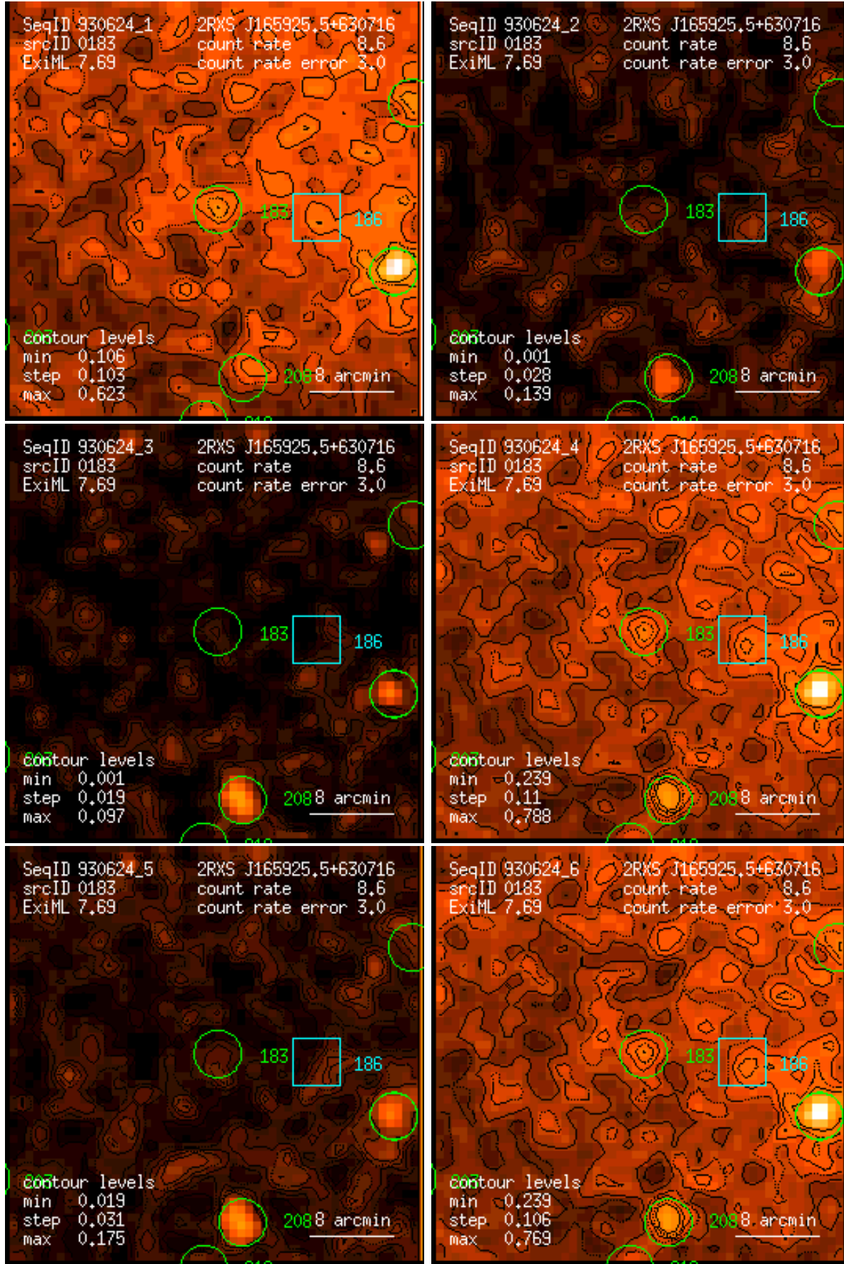
Figure 183: RASS 930624: detection 0183: band rate images, Gaussian filter: (1) PSPC channels 11 – 41, (2) 52 – 90, (3) 91 – 201, (4) 11 – 235, (5) 52 – 201, (6) 11 – 201. Broad band rates in counts/ks. Band rate contour levels in counts/ks/arcmin 2 .
