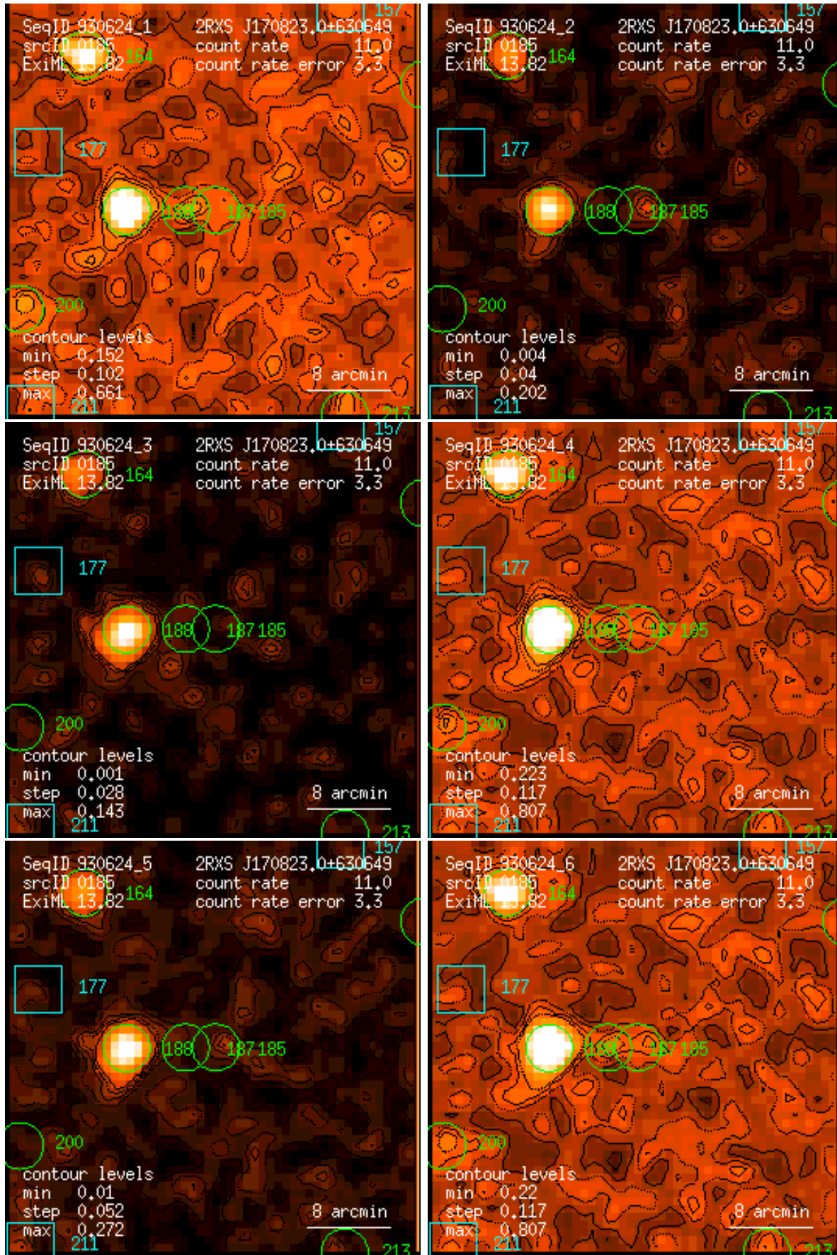
Figure 185: RASS 930624: detection 0185: band rate images, Gaussian filter: (1) PSPC channels 11 – 41, (2) 52 – 90, (3) 91 – 201, (4) 11 – 235, (5) 52 – 201, (6) 11 – 201. Broad band rates in counts/ks. Band rate contour levels in counts/ks/arcmin 2 .
