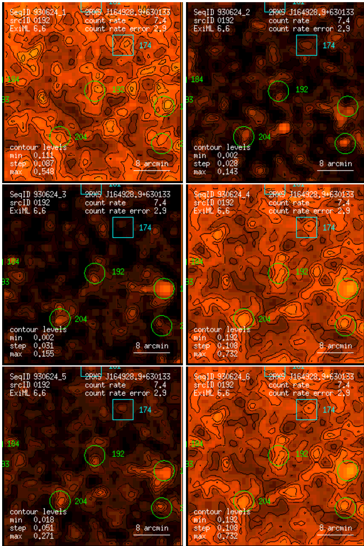
Figure 192: RASS 930624: detection 0192: band rate images, Gaussian filter: (1) PSPC channels 11 – 41, (2) 52 – 90, (3) 91 – 201, (4) 11 – 235, (5) 52 – 201, (6) 11 – 201. Broad band rates in counts/ks. Band rate contour levels in counts/ks/arcmin 2 .
