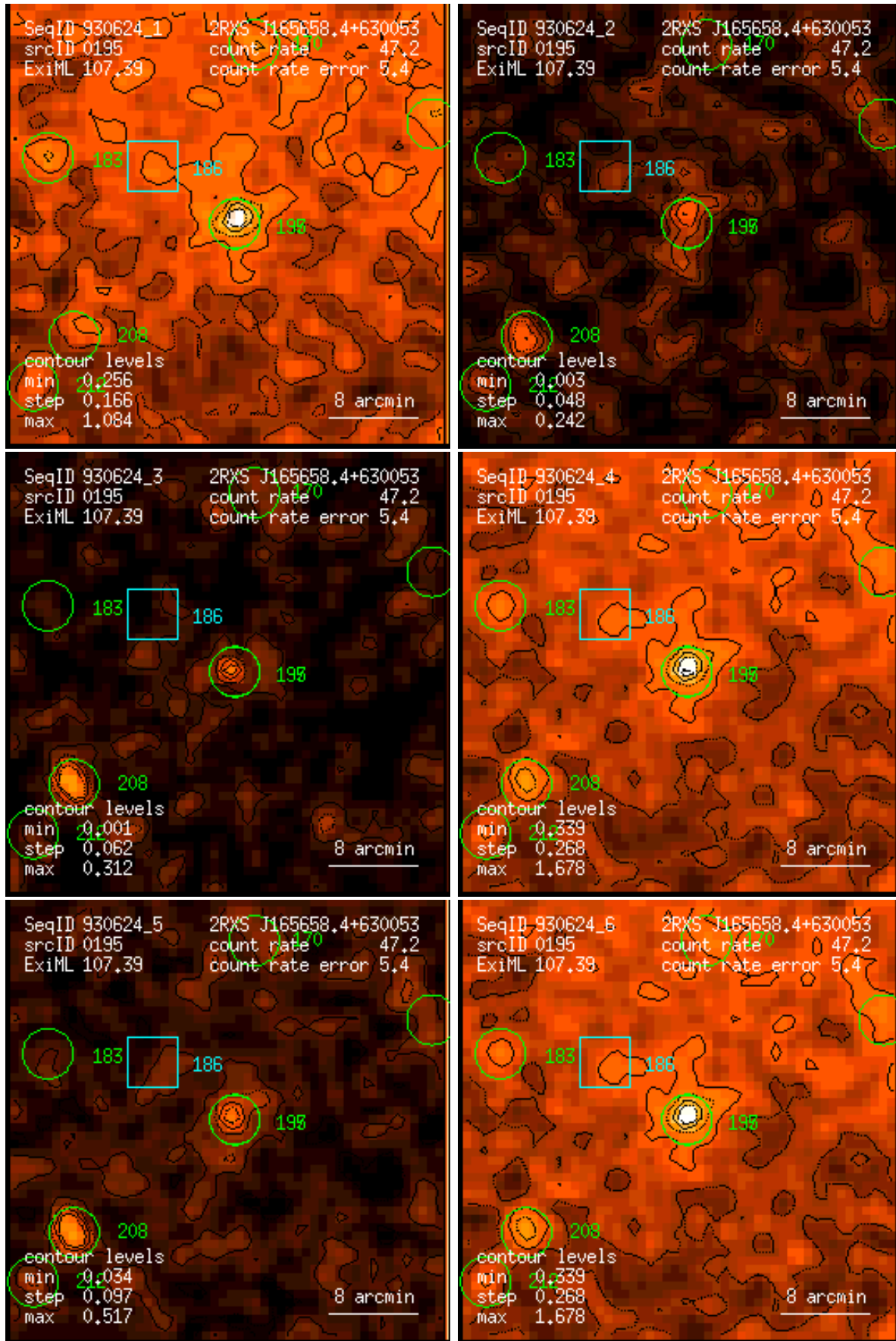
Figure 195: RASS 930624: detection 0195: band rate images, Gaussian filter: (1) PSPC channels 11 – 41, (2) 52 – 90, (3) 91 – 201, (4) 11 – 235, (5) 52 – 201, (6) 11 – 201. Broad band rates in counts/ks. Band rate contour levels in counts/ks/arcmin 2 .
