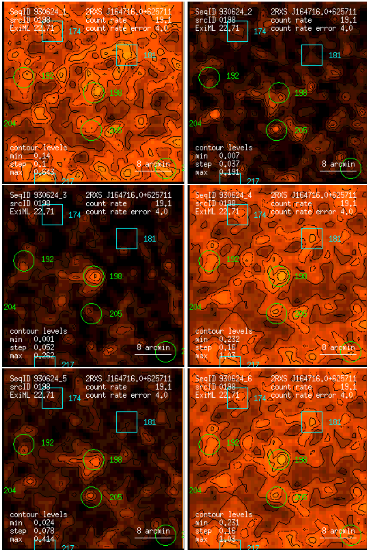
Figure 198: RASS 930624: detection 0198: band rate images, Gaussian filter: (1) PSPC channels 11 – 41, (2) 52 – 90, (3) 91 – 201, (4) 11 – 235, (5) 52 – 201, (6) 11 – 201. Broad band rates in counts/ks. Band rate contour levels in counts/ks/arcmin 2 .
