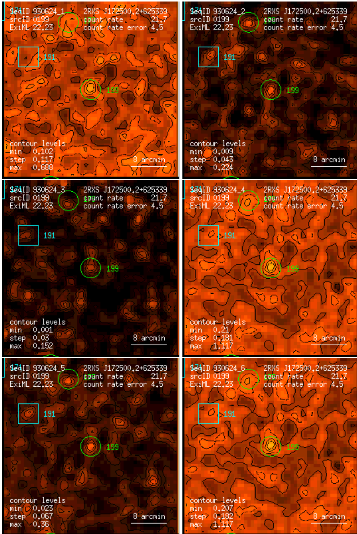
Figure 199: RASS 930624: detection 0199: band rate images, Gaussian filter: (1) PSPC channels 11 – 41, (2) 52 – 90, (3) 91 – 201, (4) 11 – 235, (5) 52 – 201, (6) 11 – 201. Broad band rates in counts/ks. Band rate contour levels in counts/ks/arcmin 2 .
