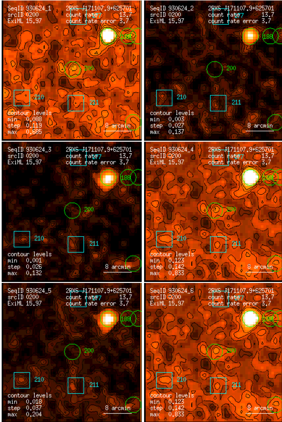
Figure 200: RASS 930624: detection 0200: band rate images, Gaussian filter: (1) PSPC channels 11 – 41, (2) 52 – 90, (3) 91 – 201, (4) 11 – 235, (5) 52 – 201, (6) 11 – 201. Broad band rates in counts/ks. Band rate contour levels in counts/ks/arcmin 2 .
