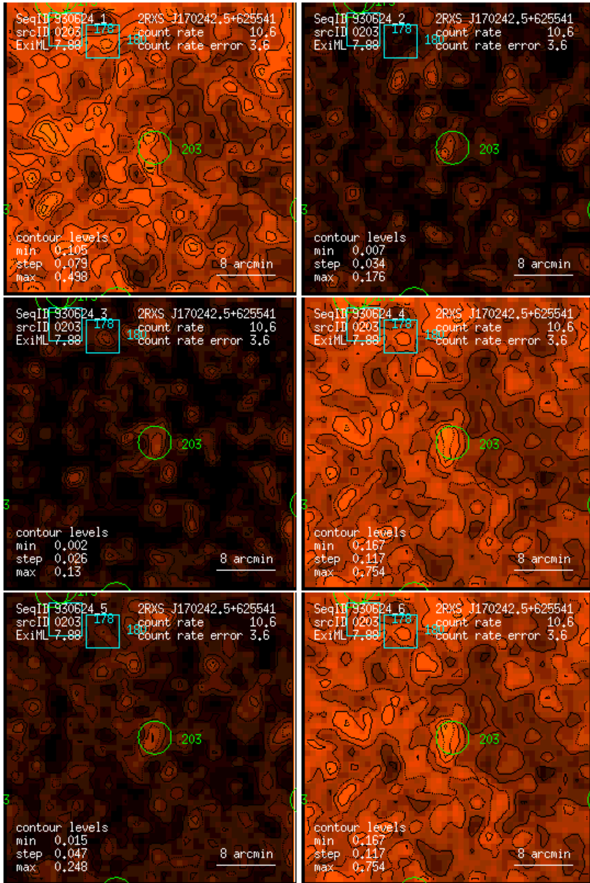
Figure 203: RASS 930624: detection 0203: band rate images, Gaussian filter: (1) PSPC channels 11 – 41, (2) 52 – 90, (3) 91 – 201, (4) 11 – 235, (5) 52 – 201, (6) 11 – 201. Broad band rates in counts/ks. Band rate contour levels in counts/ks/arcmin 2 .
