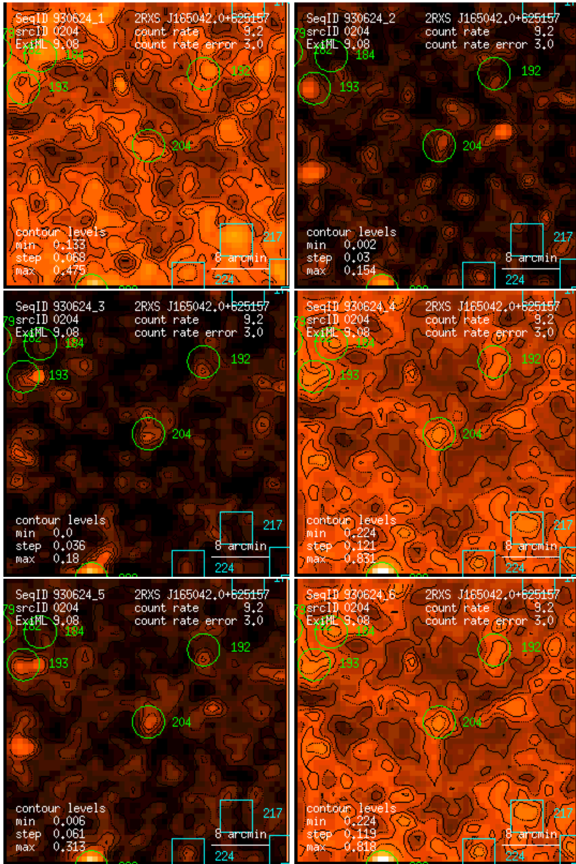
Figure 204: RASS 930624: detection 0204: band rate images, Gaussian filter: (1) PSPC channels 11 – 41, (2) 52 – 90, (3) 91 – 201, (4) 11 – 235, (5) 52 – 201, (6) 11 – 201. Broad band rates in counts/ks. Band rate contour levels in counts/ks/arcmin 2 .
